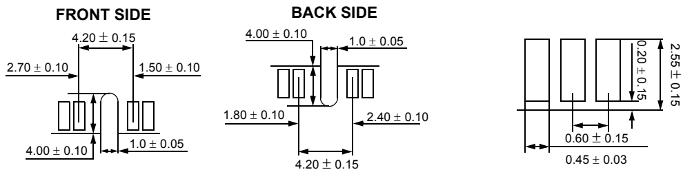
DETAIL a
