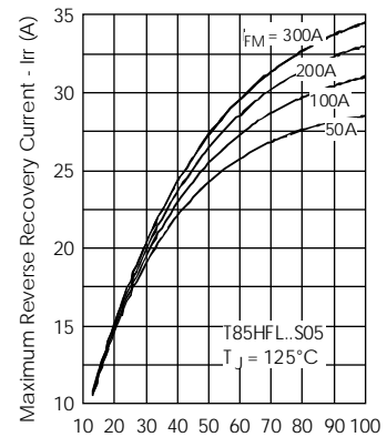
Fig. 33 - Recovery Current Characteristics
