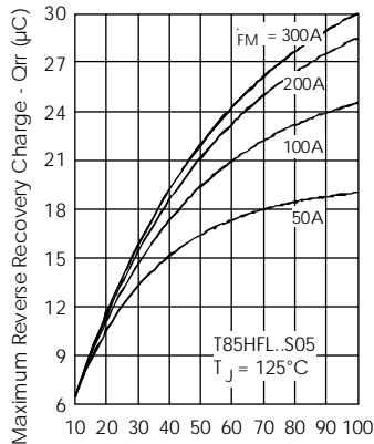
Fig. 32 - Recovery Charge Characteristics
