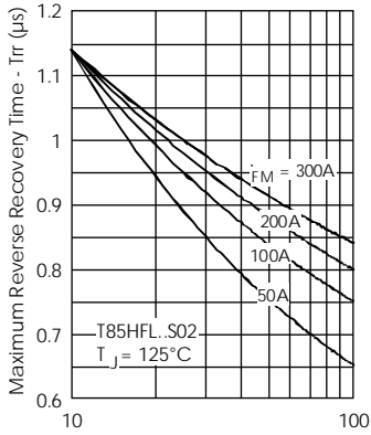
Fig. 28 - Recovery Time Characteristics
