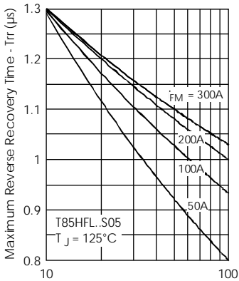
Fig. 31 - Recovery Time Characteristics
