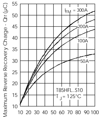
Fig. 35 - Recovery Charge Characteristics
