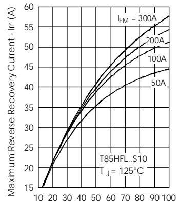
Fig. 36 - Recovery Current Characteristics
