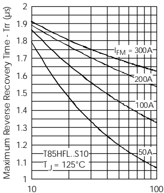
Fig. 34 - Recovery Time Characteristics
