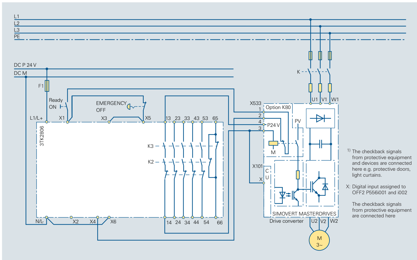
Circuit diagram 6/70 Stop Category 0, single-channel, with feedback circuit. Category 3 acc. to EN 954-1 function with motor which is coasting down
