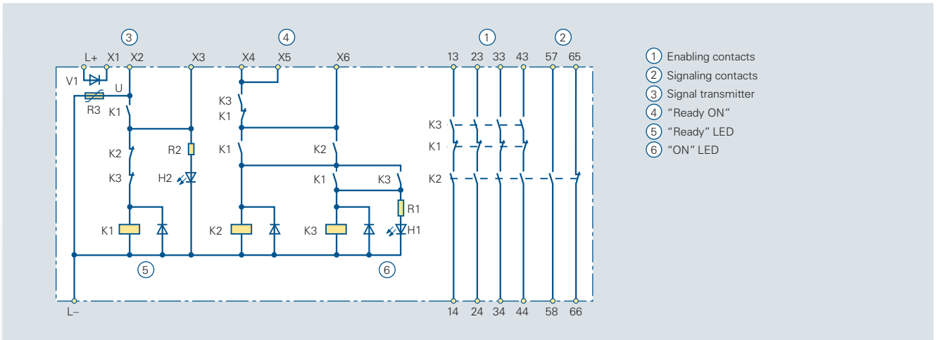
Circuit diagram 6/12 Internal circuit diagram of a 3TK28 04 contactor safety combination (DC operation)
