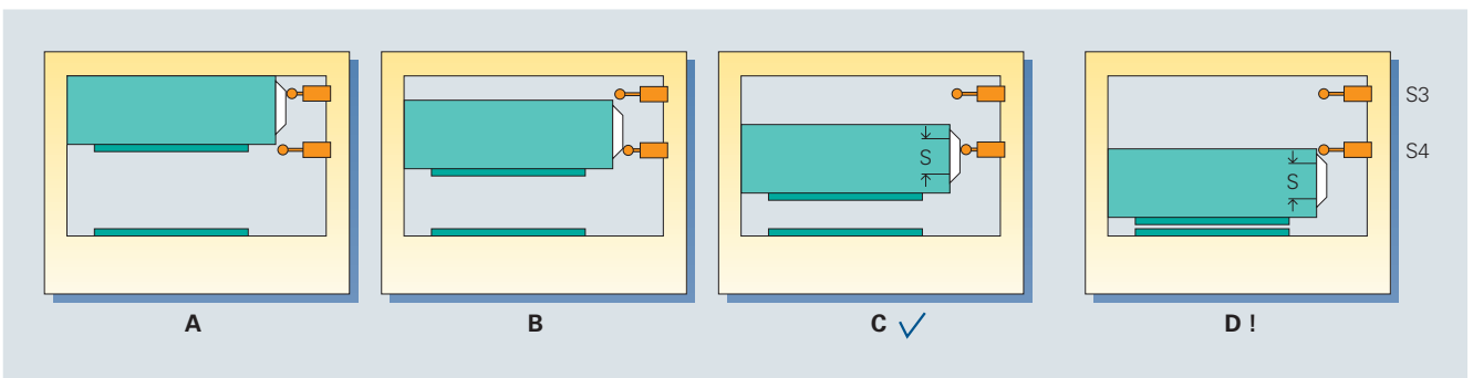
Fig. 6/4 Function schematic of the press control. The permissible overtravel "s" corresponds to the length of the cam which actuates position switch S4. According to ZH 1/456, the press manufacturer must define "s."
