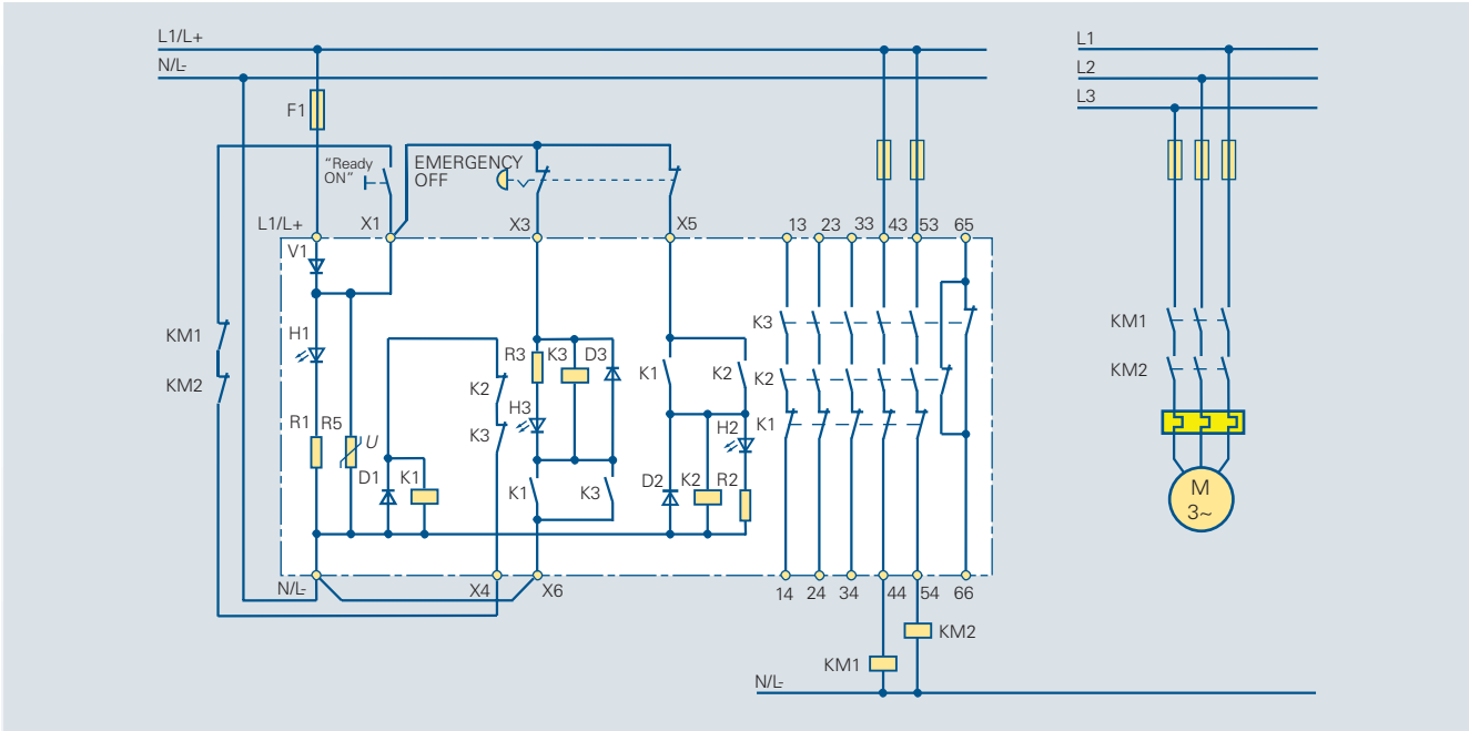
Circuit diagram 6/15 Contactor safety combination 3TK28 06 for a two-channel EMERGENCY OFF circuit. This circuit can also be used for the 3TK28 05 (Cat. 3).
