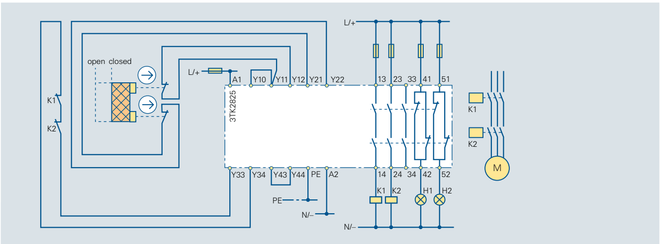
Circuit diagram 6/45 3TK2825 for protective door monitoring with 2 SIGUARD position switches, autostart, Category 4 acc. to EN 954-1, two-channel, with feedback circuit
