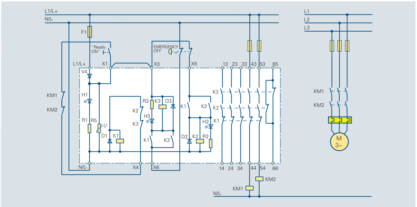
Circuit diagram 6/16 Contactor safety combination 3TK28 06 for a two-channel EMERGENCY OFF circuit with cross-circuit protection. This circuit can also be used for the 3TK28 05 (Cat. 4).
