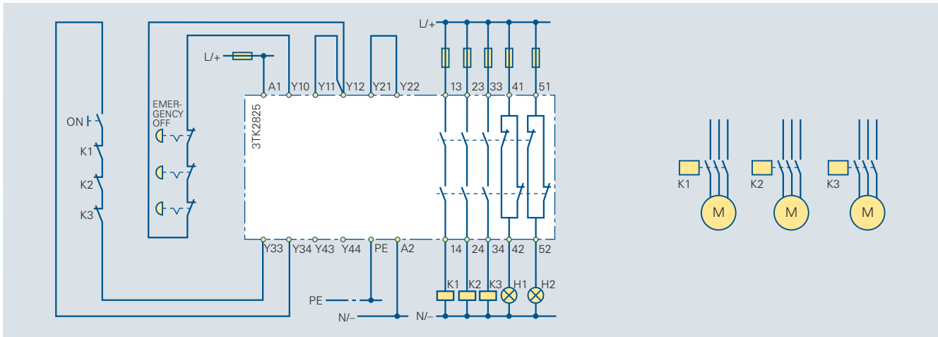
Circuit diagram 6/33 3TK2825 EMERGENCY OFF, Category 2, single-channel, according to EN 954-1, monitored start
