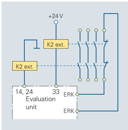
Circuit diagram 6/60
