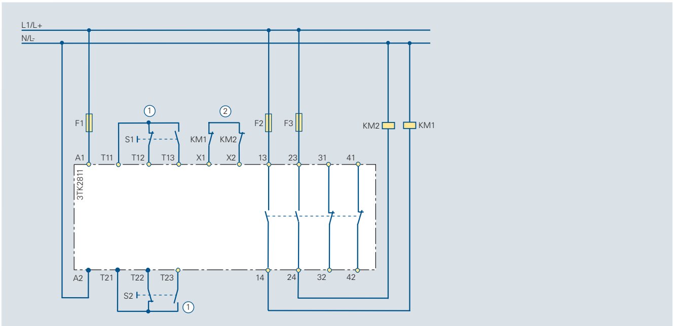
Circuit diagram 6/25 Two-hand control device 3TK28 11
