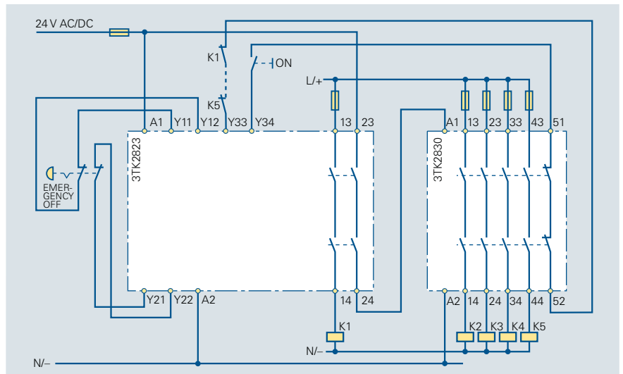
Circuit diagram 6/37 3TK2823 expanded with 3TK2830 for EMERGENCY OFF, Category 4 acc. to EN 954-1, two-channel, with feedback circuit
