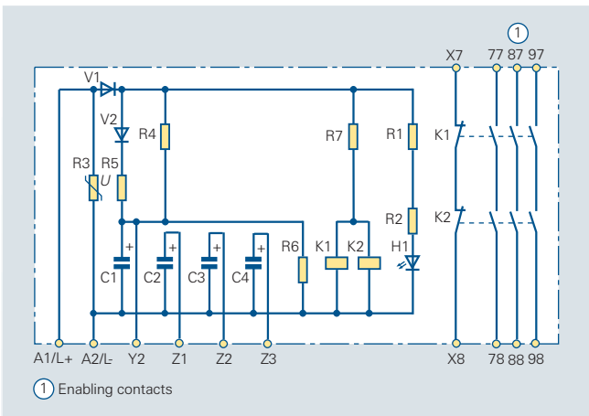
Circuit diagram 6/23 Internal circuit diagram of a contactor safety combination delay module 3TK29 23, 43, 83 (DC operation)
