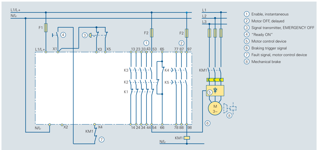
Circuit diagram 6/18 Contactor safety combination 3TK28 07 for controlled actuation of EMERGENCY OFF.
