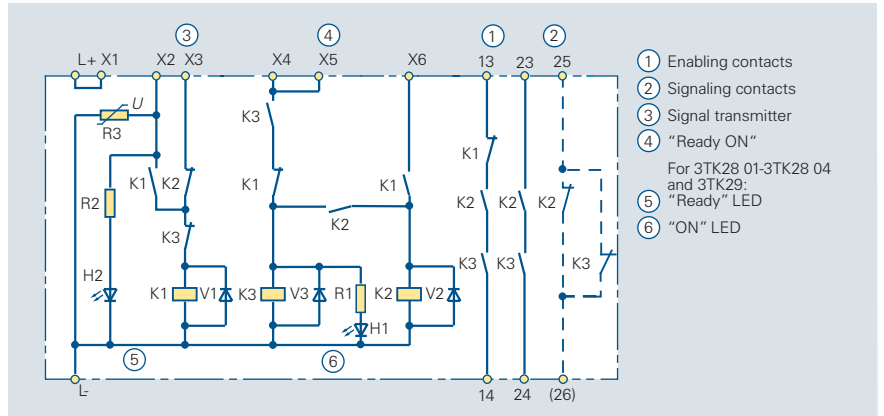
Circuit diagram 6/8 Internal circuit diagram of 3TK28 01, 3TK28 02 contactor safety combination (DC operation) NC signaling contact for 3TK28 02. For 3TK 2801/02, terminals "X2, X4, X6" are at the top, for TK 2803, there is no terminal "X3"
