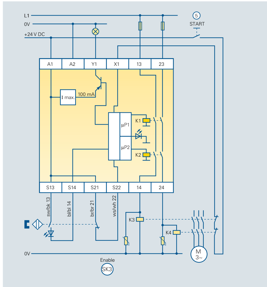
Circuit diagram 6/49 SIGUARD magnetically-operated switch with evaluation unit 3SE6801-1CC for Category 3 acc. to EN 954-1
