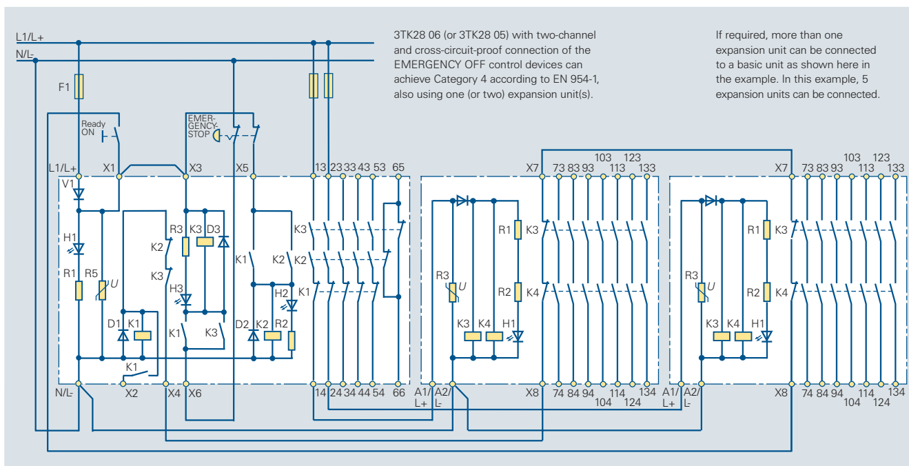
Circuit diagram 6/21 Contactor safety combinations 3TK28 06 for two-channel and cross-circuit-proof connection of the EMERGENCY OFF control device and two 3TK29 07 expansion units. This circuit can also be realized using the 3TK28 05 unit.
