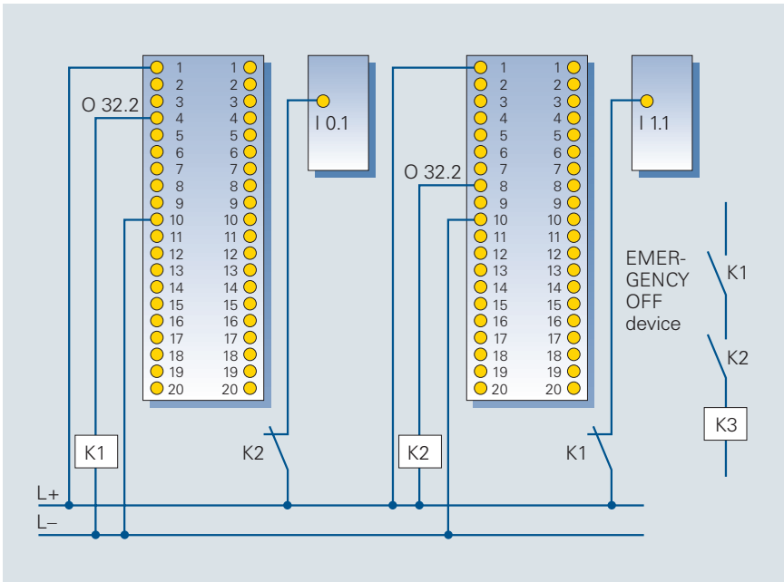
Circuit diagram 6/65 Controlling redundant auxiliary contactors with checkback signals via positively-driven auxiliary contacts
