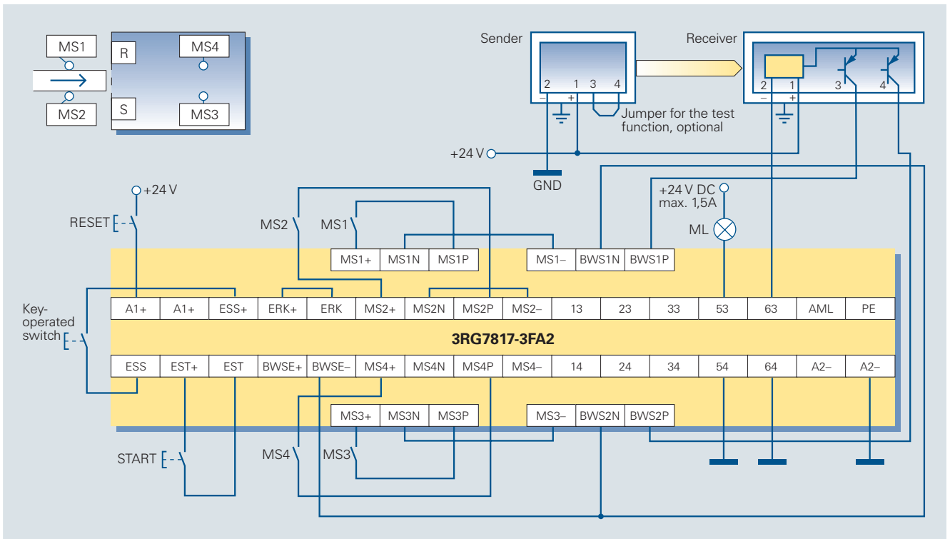
Circuit diagram 6/59 Connecting-up the muting evaluation unit using the muting function
