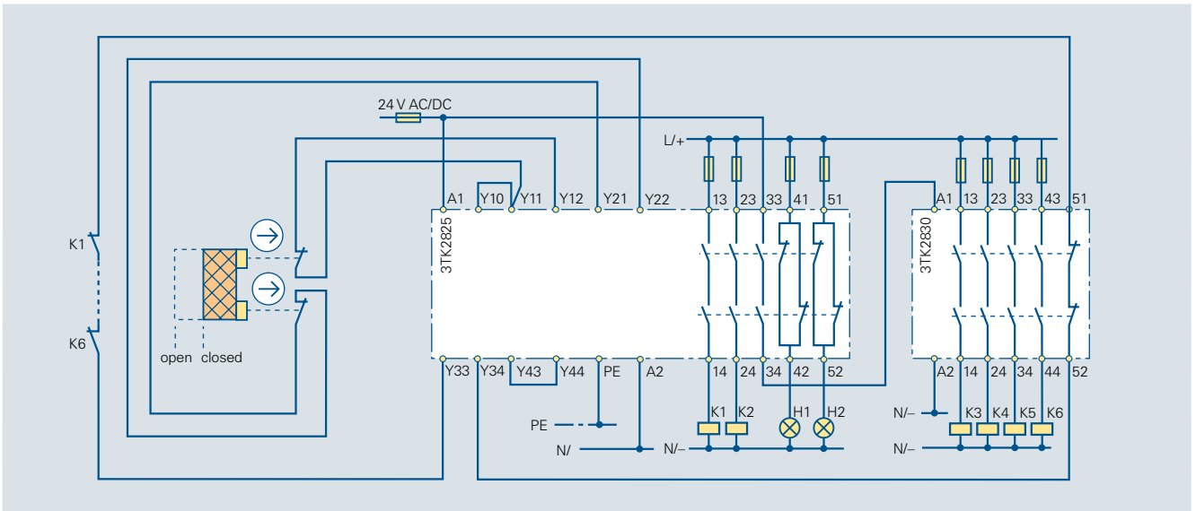
Circuit diagram 6/48 3TK2825 expanded by 3TK2830 for protective door monitoring with 2 SIGUARD position switches, Category 4 acc. to EN 954-1, two-channel, with feedback circuit, autostart
