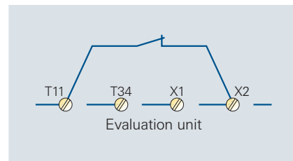
Circuit diagram 6/56 Automatic restart
