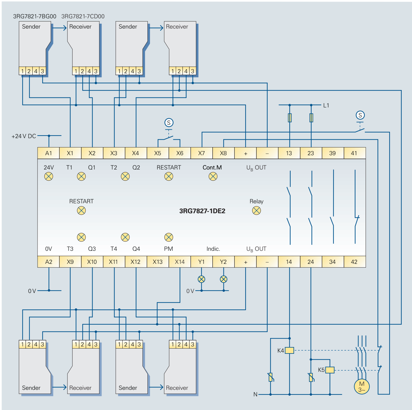
Circuit diagram 6/62
