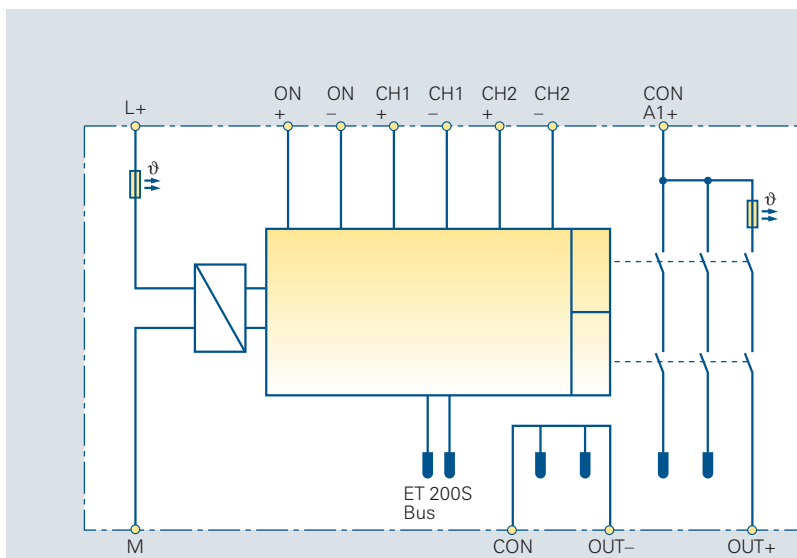
Circuit diagram 6/67 EMERGENCY OFF with monitored start, Category 4
