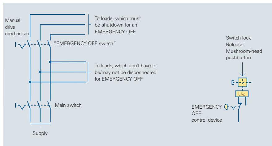
Circuit diagram 6/1 EMERGENCY OFF switch with manual actuation or remote actuation via undervoltage release
