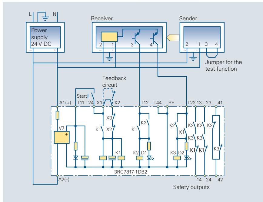
Circuit diagram 6/55 Connecting-up the standard evaluation unit for SIGUARD light curtains
