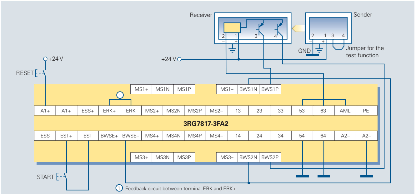
Circuit diagram 6/58 Connecting-up the muting evaluation unit without using the muting function
