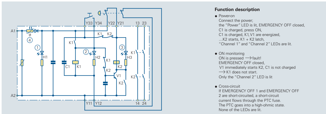
Circuit diagram 6/28 Function description 3TK2823
