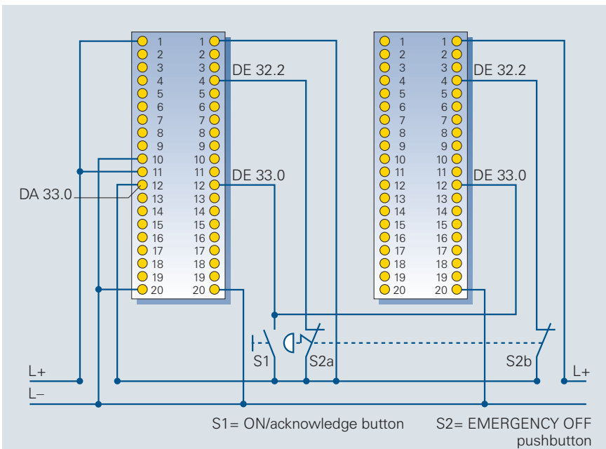
Circuit diagram 6/66 Connecting the ON/acknowledge button and the EMERGENCY OFF control devices with cross-circuit monitoring
