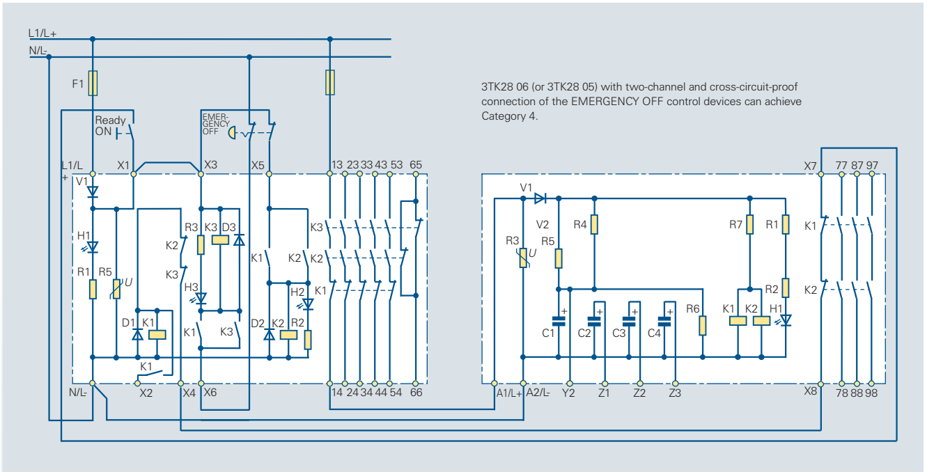
Circuit diagram 6/22 Contactor safety combination 3TK28 06 for two-channel and cross-circuit-proof connection of the EMERGENCY OFF control device and a 3TK29 . 3 expansion unit. This circuit can also be used with the 3TK28 05.
