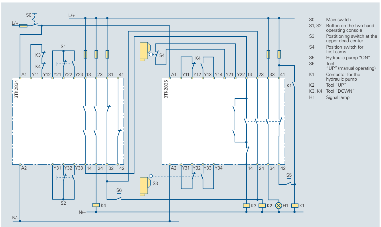
Circuit diagram 6/54 3TK2834 two-hand control device in conjunction with a 3TK2835 overtravel tester to monitor the overtravel in linear hydraulic-, pneumatic- and spindle presses acc. to VBG 7 n 5.2 § 11, Category 4 acc. to EN 954-1
