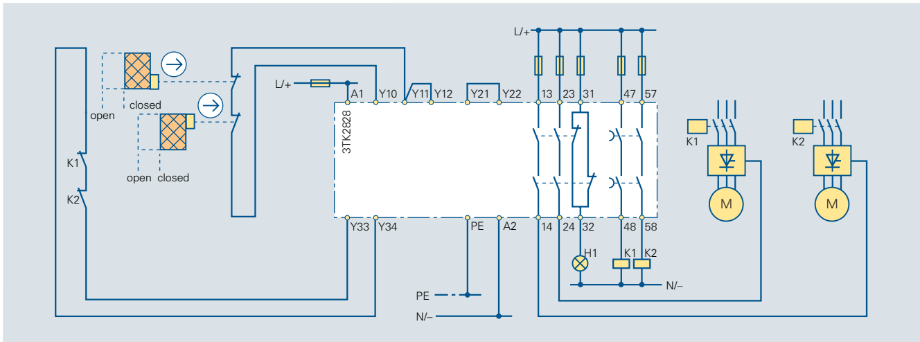
Circuit diagram 6/46 3TK2828 for protective door monitoring (2 protective doors are cascaded, each with 1 SIGUARD position switch), stop Category 1, Category 2 acc. to EN 954-1, single-channel, with feedback circuit, autostart
