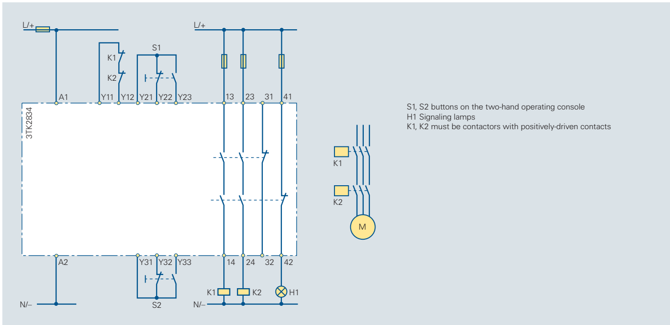
Circuit diagram 6/52 3TK2834 two-hand control device, Category 4 acc. to EN 954-1
