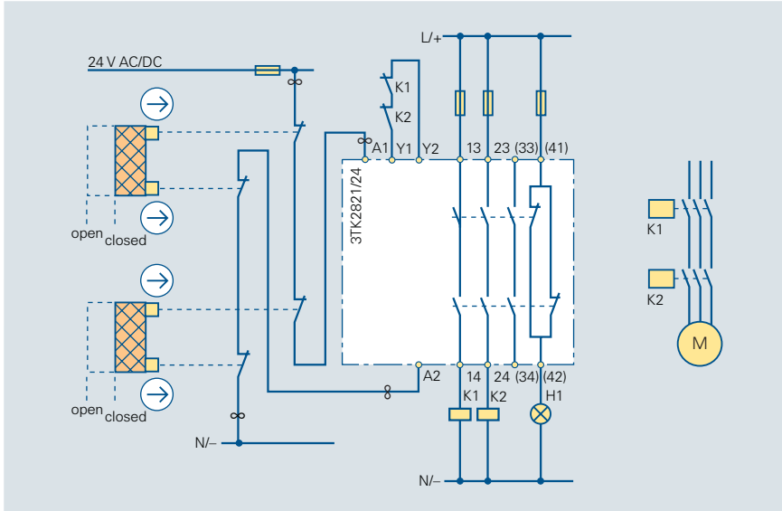
Circuit diagram 6/42 3TK2821/24 for protective door monitoring (2 protective doors are cascaded, each with 2 SIGUARD position switches), Category 3(4) acc. to EN 954-1, two-channel with feedback circuit, autostart, ∞ for Category 4 – the cable has to be routed so that it is especially protected)
