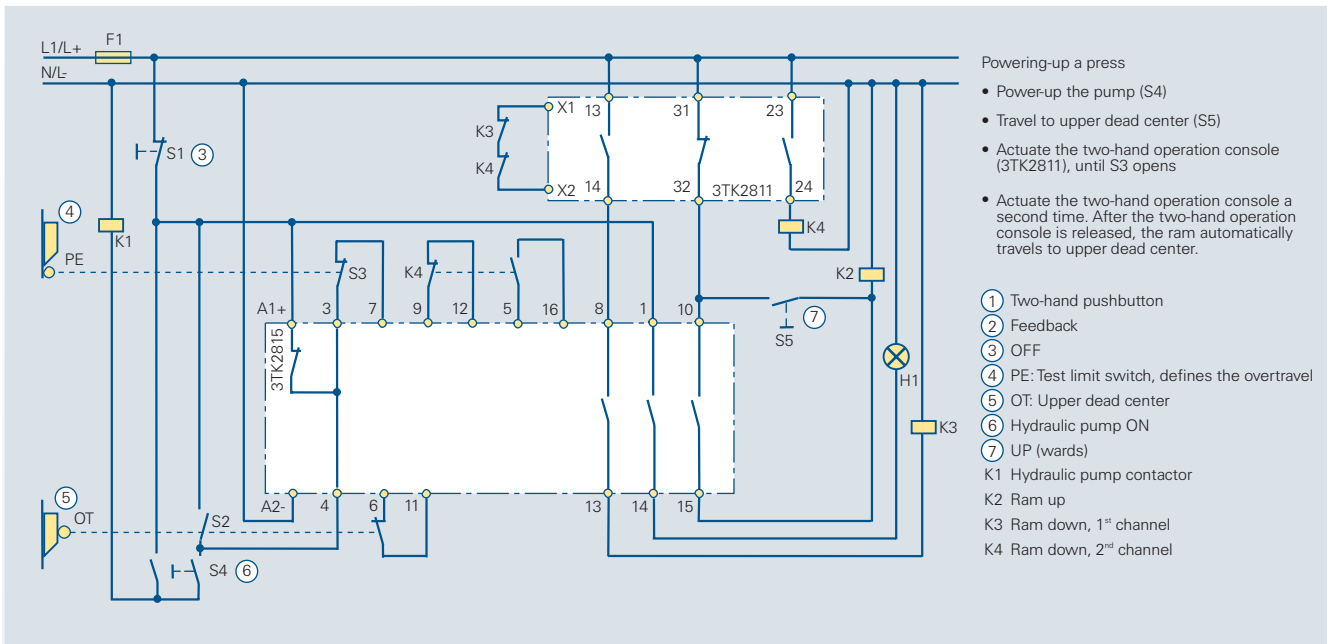
Circuit diagram 6/26 Overtravel tester 3TK28 15 and two-hand control device 3TK28 11
