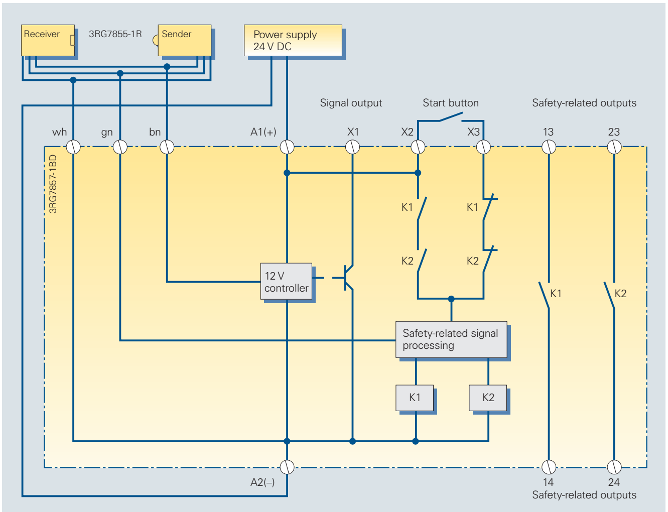
Circuit diagram 6/63
