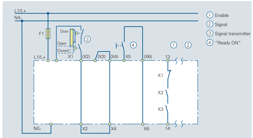
Circuit diagram 6/10
