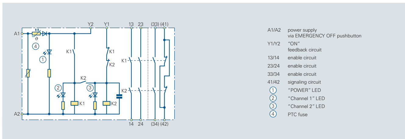
Circuit diagram 6/29 Internal circuit diagram of the 3TK2821/24
