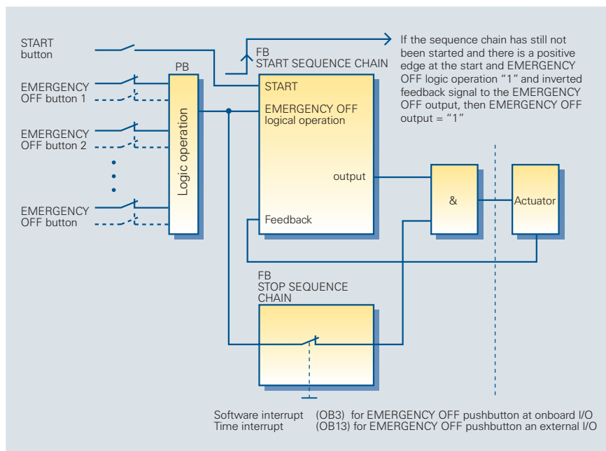
Circuit diagram 6/64 Principle of identifying and shutting down EMERGENCY OFF sequence chains for fail-safe S5-95F PLC
