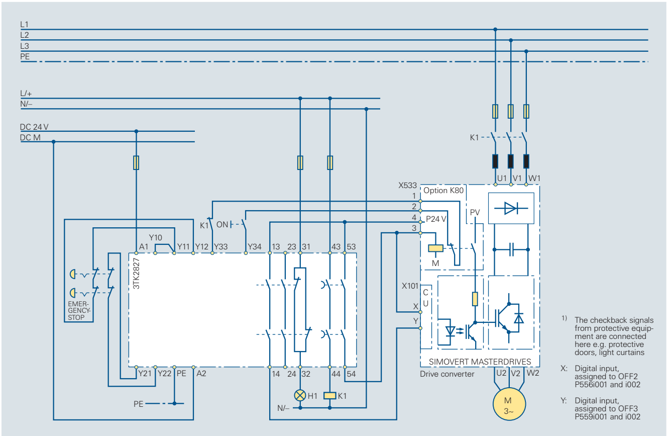
Circuit diagram 6/73 Stop Category 1, two-channel, with feedback circuit. Category 3 acc. to EN 954-1. Function with controlled motor stop along the torque limit.
