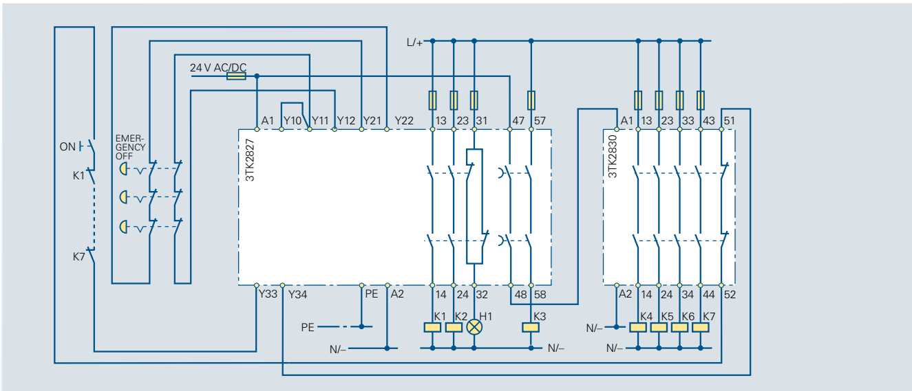
Circuit diagram 6/39 3TK2827 expanded by 3TK2830 for EMERGENCY OFF, Category 4, two-channel, monitored start
