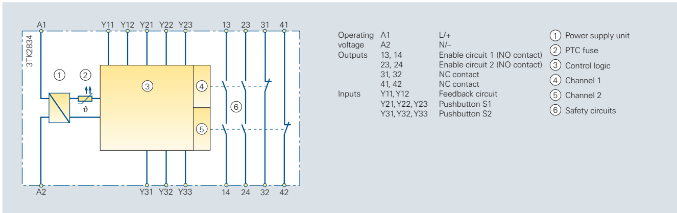
Circuit diagram 6/51 Internal circuit diagram of the 3TK2834 two-hand control device
