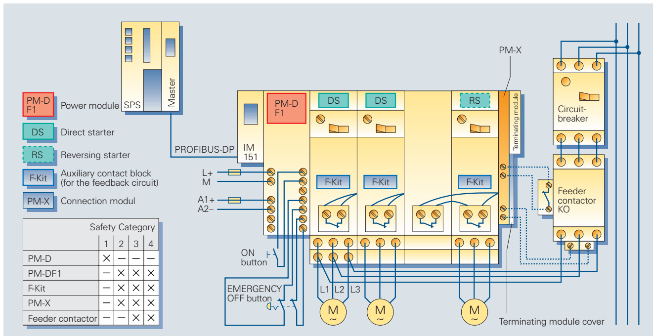
Circuit diagram 6/67 EMERGENCY OFF with monitored start, Category 4
