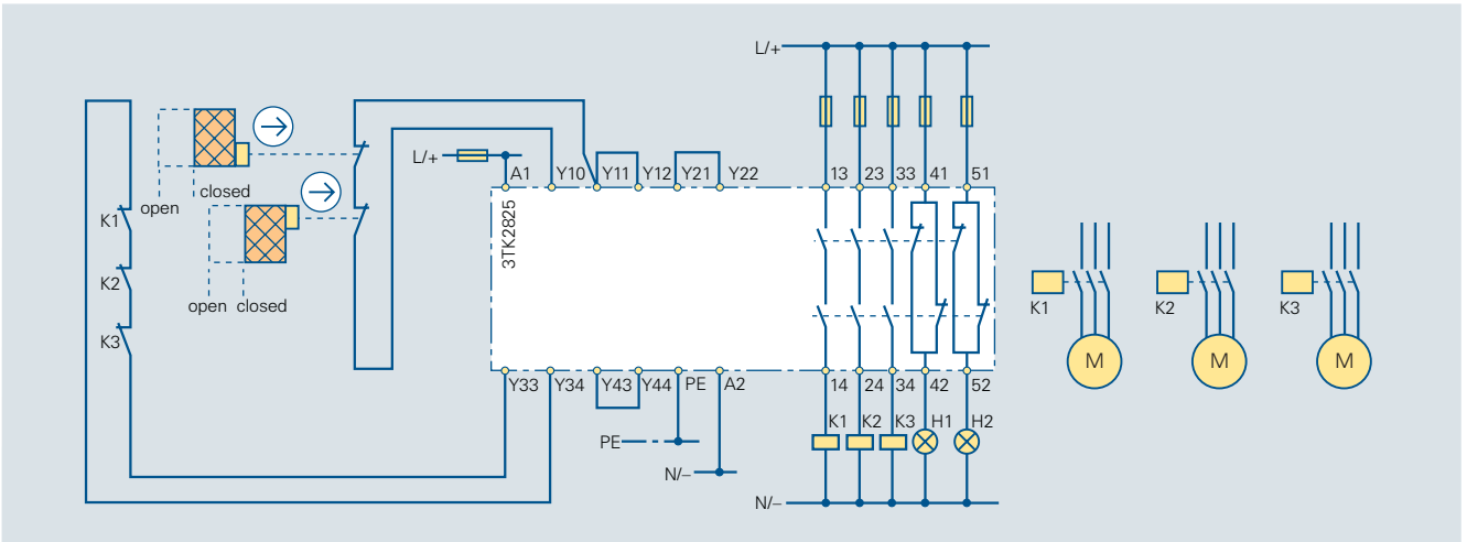
Circuit diagram 6/44 3TK2825 for protective door monitoring (2 protective doors are cascaded, each with 1 SIGUARD position switch), autostart, Category 2 acc. to EN 954-1, single-channel, with feedback circuit
