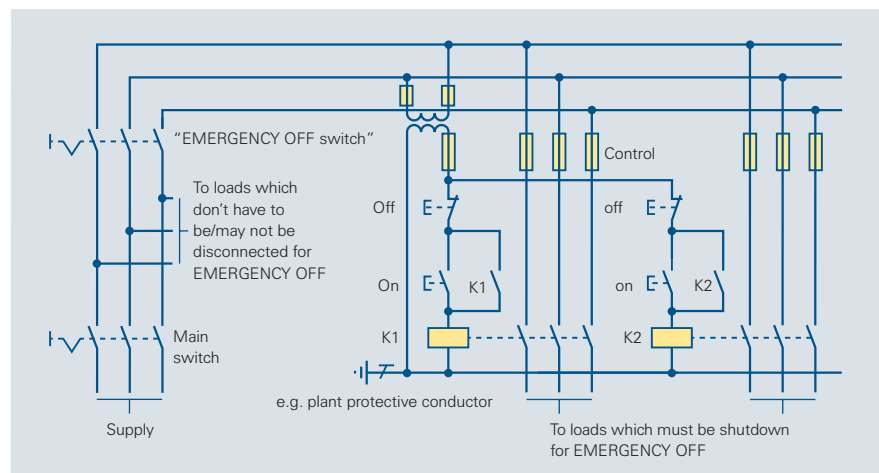
Circuit diagram 6/2 Example of a machine control with EMERGENCY OFF switch (this is only permissible with some restrictions)
