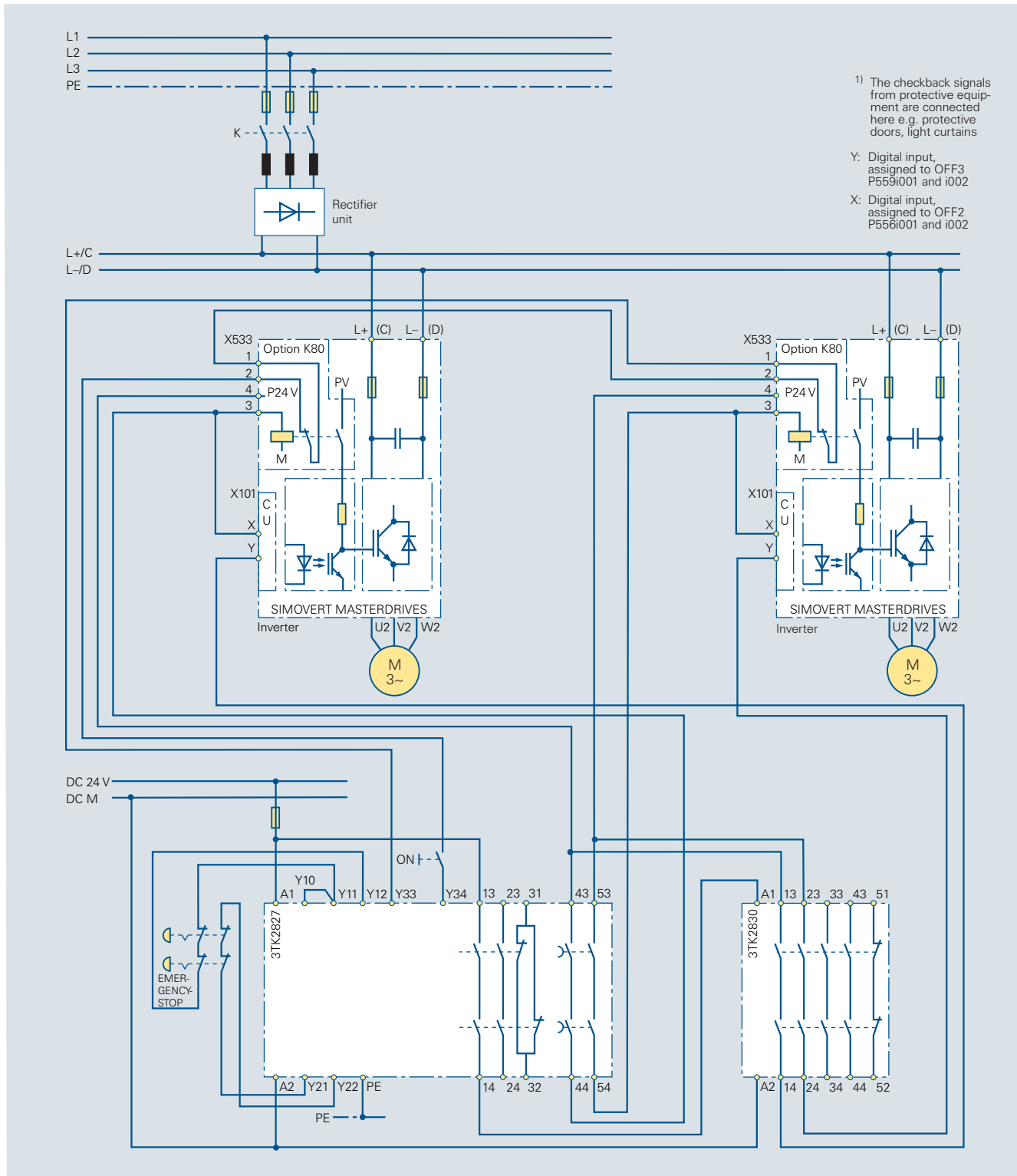
Circuit diagram 6/72
