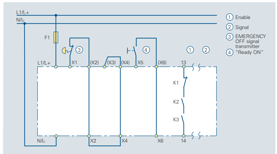
Circuit diagram 6/9 Contactor safety combinations 3TK28 01 to 3TK2804 for EMERGENCY OFF circuits
