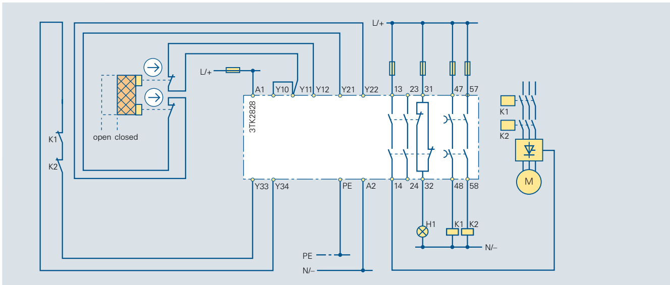
Circuit diagram 6/47 3TK2828 for protective door monitoring with 2 SIGUARD position switches, stop Category 1, Category 3 acc. to EN 954-1, two-channel, with feedback circuit, autostart
