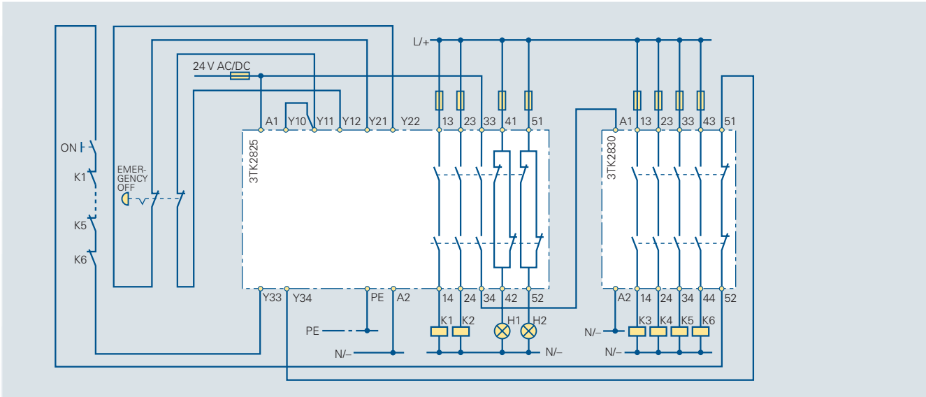
Circuit diagram 6/38 3TK2825 expanded by 3TK2830 for EMERGENCY OFF, Category 4 acc. to EN 954-1, two-channel acc. to EN 954-1, monitored start
