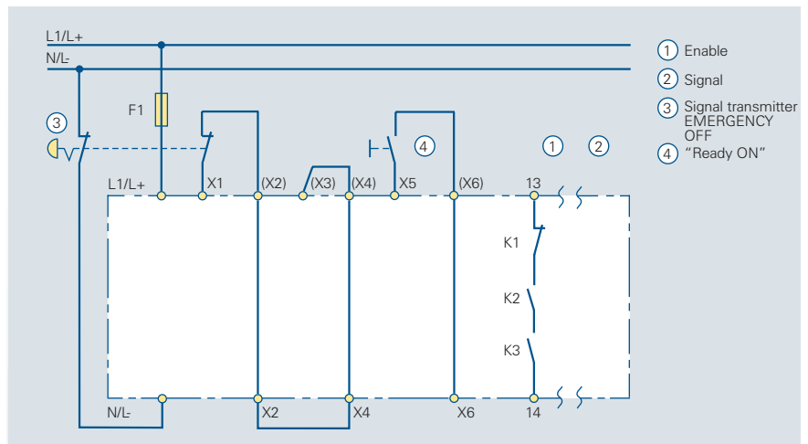
Circuit diagram 6/11
