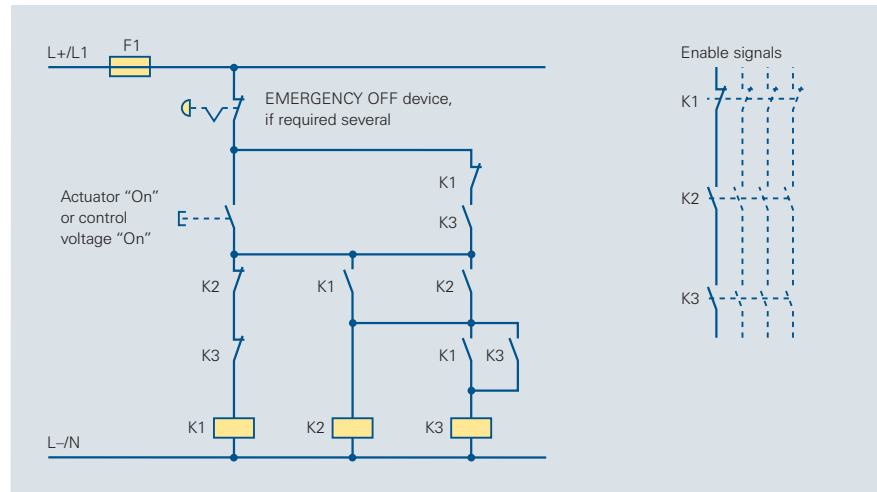
Circuit diagram 6/5 Contactor combination using three auxiliary contactors with self-monitoring, single-channel
