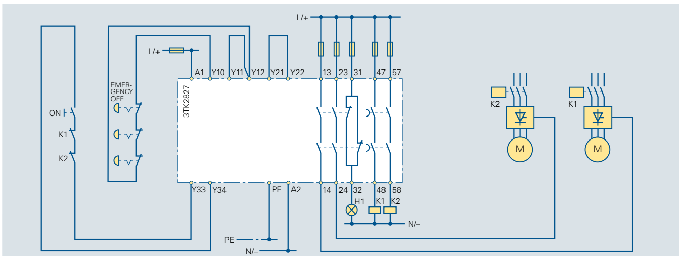
Circuit diagram 6/35 3TK2827 EMERGENCY OFF, Category 2, single-channel, according to EN 954-1, monitored start
