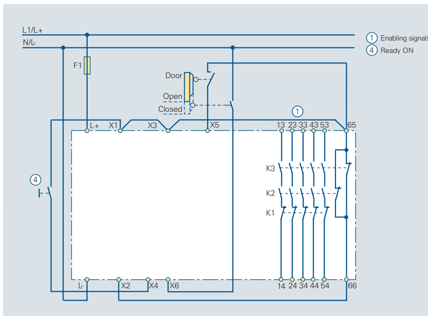
Circuit diagram 6/19 Contactor safety combination 3TK28 06 to monitor moving protective devices
