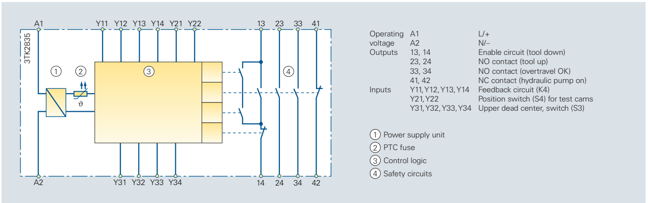
Circuit diagram 6/53 Internal circuit diagram of the 3TK2835 overtravel tester
