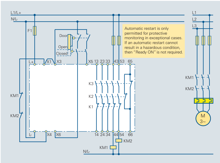
Circuit diagram 6/20 Contactor safety combination 3TK28 06 for two-channel and cross-circuit proof monitoring of moving protective devices with automatic restart
