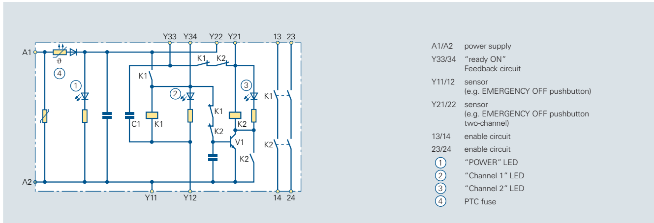
Circuit diagram 6/27 Internal circuit diagram of the 3TK2823
