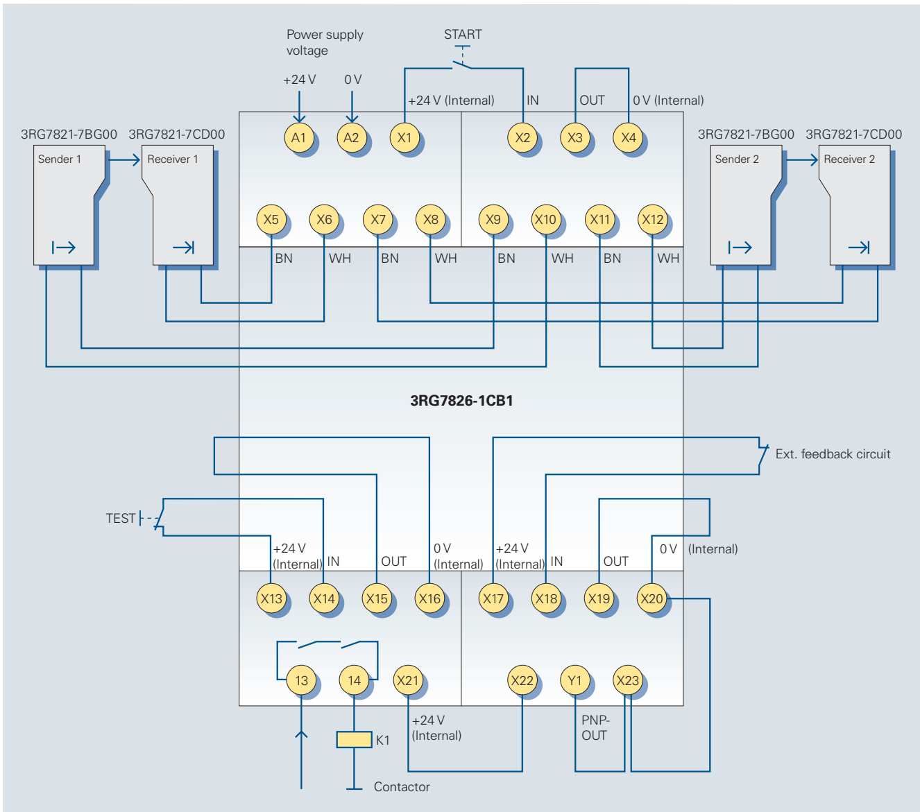
Circuit diagram 6/61
