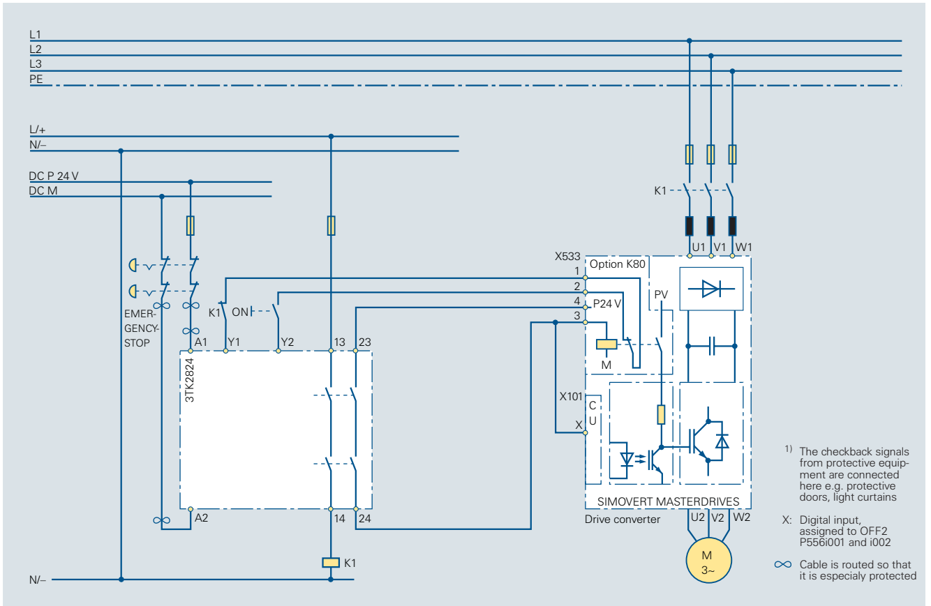
Circuit diagram 6/71 Stop Category 0, two-channel, with feedback circuit. Category 3 acc. to EN 954-1. Function with motor which is coasting down
