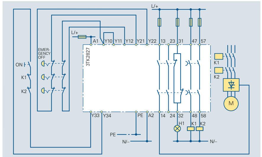
Circuit diagram 6/36 3TK2827 EMERGENCY OFF with shut-down, stop Category 1, for Category 3 according to EN 954-1, two-channel, with feedback circuit, monitored start
