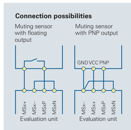
Circuit diagram 6/57 Connecting different muting sensors
