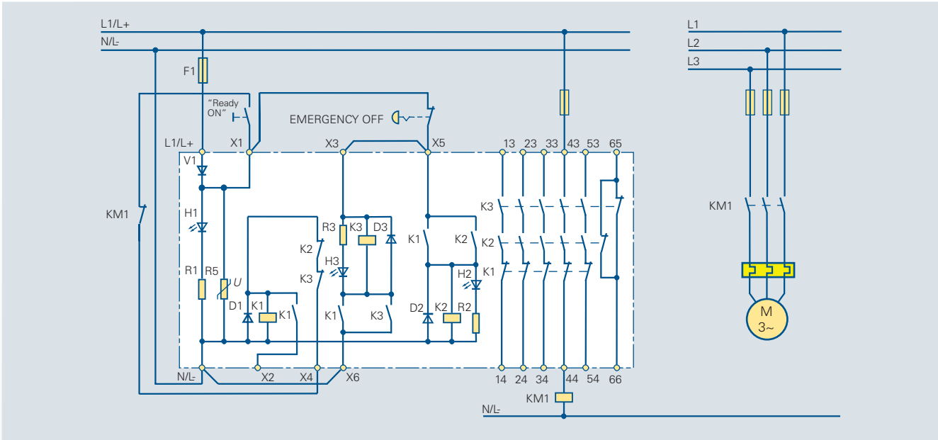
Circuit diagram 6/14 Contactor safety combination 3TK28 06 for a single-channel EMERGENCY OFF circuit. This circuit can also be used for the 3TK28 05 (Cat. 2).
