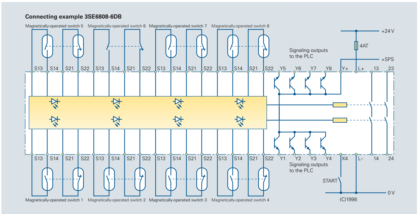
Circuit diagram 6/50
