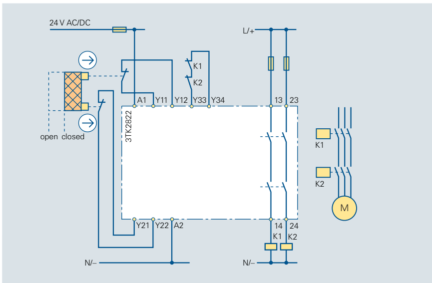
Circuit diagram 6/43 3TK2822 for protective door monitoring (2 protective doors are cascaded, each with 1 SIGUARD position switch), Category 4 acc. to EN 954-1, two-channel with feedback circuit, autostart
