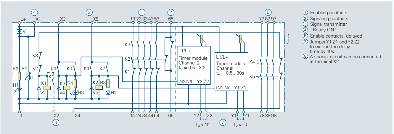
Circuit diagram 6/17 Internal circuit diagram of a 3TK28 07 contactor safety combination (DC operation)
