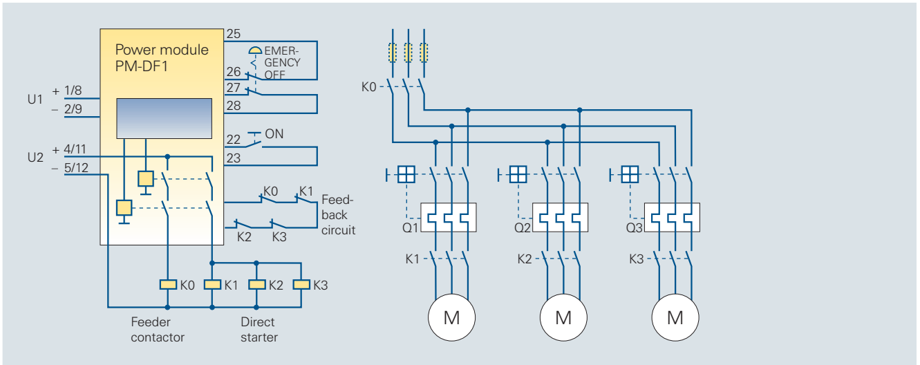
Circuit diagram 6/69 Monitoring load feeders, EMERGENCY OFF, stop Category 0, monitored start, Category 4. The load feeders are monitored, as the contactor NC contacts (F kit) are switched as "feedback circuits" in series with the ON button.
