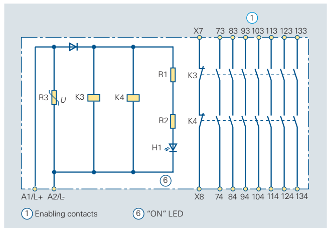
Circuit diagram 6/24 Internal circuit diagram of a contactor safety combination supplementary module 3TK29 07 (DC operation)
