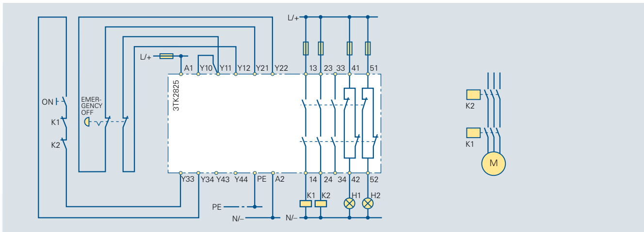
Circuit diagram 6/34 3TK2825 EMERGENCY OFF, Category 4, two-channel, according to EN 954-1, monitored start
