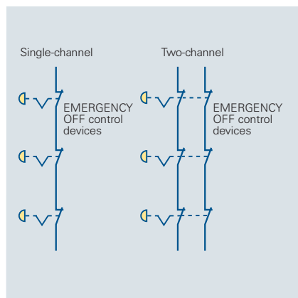
Circuit diagram 6/6 Several EMERGENCY OFF control devices
