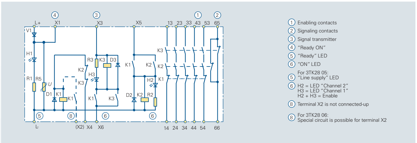
Circuit diagram 6/13 Internal circuit diagram of a 3TK28 05, 3TK28 06 contactor safety combination (DC operation); terminal X2 is only connected-up for the 3TK28 06 device
