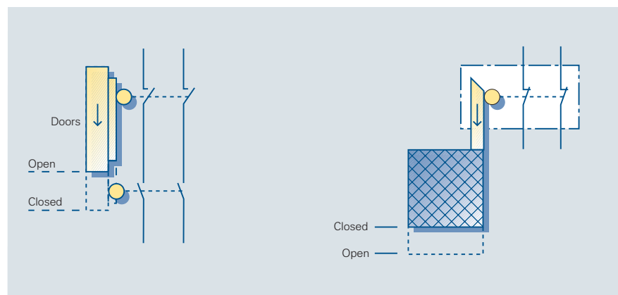
Circuit diagram 6/7 SIGUARD position switches used to monitor moving protective equipment
