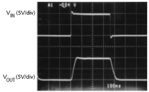
FIGURE 2. The LM6172 Driving a 510 pF Load with a 30 \Omega Isolation Resistor
