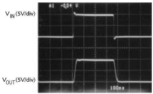
FIGURE 3. The LM6172 Driving a 220 pF Load with a 50 \Omega Isolation Resistor
