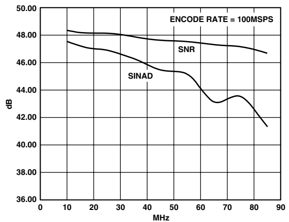
TPC 6. SINAD/SNR vs. A_{IN} Frequency
