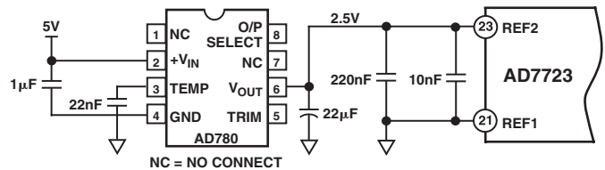
Figure 21. External Reference Circuit Connection
