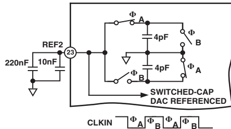
Figure 20. REF2 Equivalent Input Circuit
