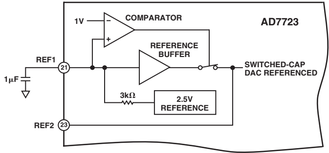
Figure 19. Reference Circuit Block Diagram
