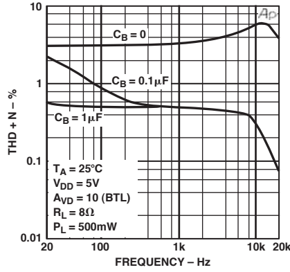
TPC 2. THD+N vs. Frequency
