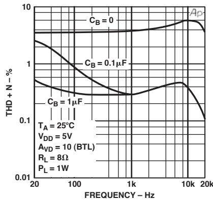
TPC 5. THD+N vs. Frequency
