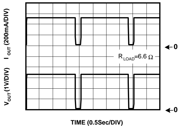
Overtemperature Shutdown
